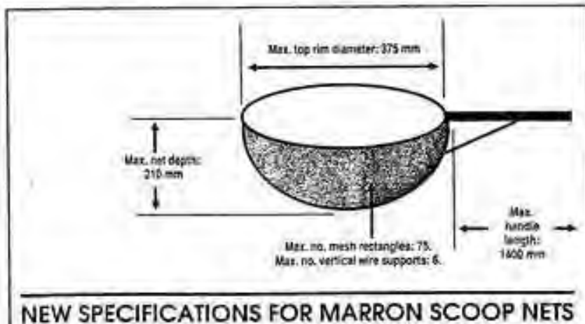
New legal marron fishing gear (not to scale). For more information contact the Fisheries Department.
